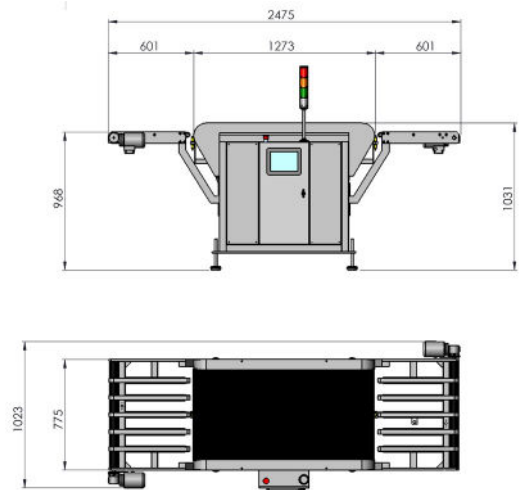
Erizo 100 + 2 Conveyors
